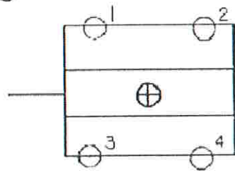
Typical Spacing of Percolation Test Holes on Proposed Absorption Fields
