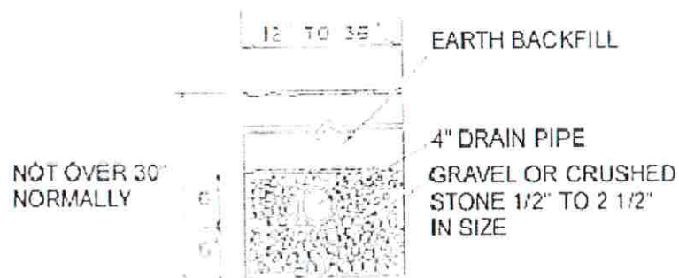
CROSS SECTION OF ABSORPTION TRENCH
